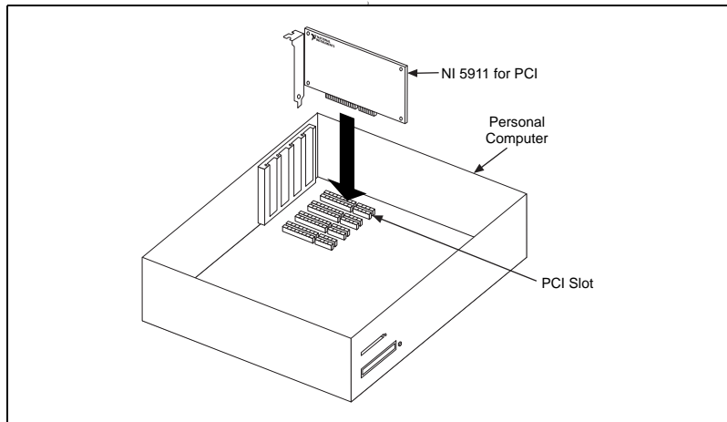
Figure 1. Installing the NI 5911 for PCI
